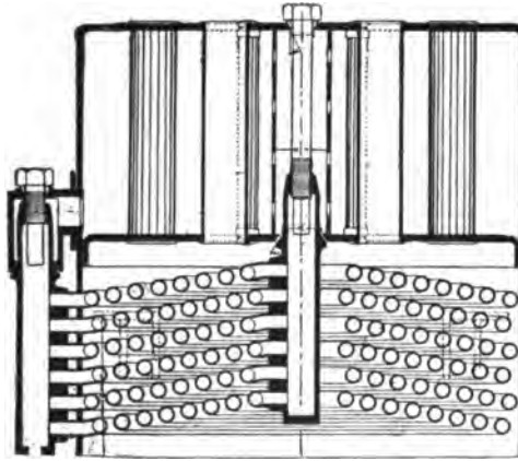
FIG. 160.—The Geneva Carriage Boiler. This boiler consists of several coils of tubing connected at inner and outer extremities to headers, as shown. The water and steam chamber above is constructed like an ordinary flue boiler.
